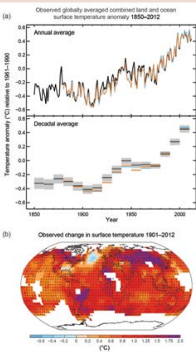
(a) Observed global mean combined land and ocean surface temperature anomalies from 1850 to 2012 from three data sets. Top panel: annual mean values. Bottom panel: decadal mean values including the estimate of uncertainty for one dataset (black). Anomalies are relative to the mean of 1961–1990. (b) Map of the observed surface temperature change from 1901 to 2012 derived from temperature trends determined by linear regression from one dataset (orange line in panel a). (From http://www.ipcc.ch/pdf/assessment-report/ar5/wg1/WG1AR5_SPM_FINAL.pdf Summary for Policy makers, IPCC report 5th, 2013.)
