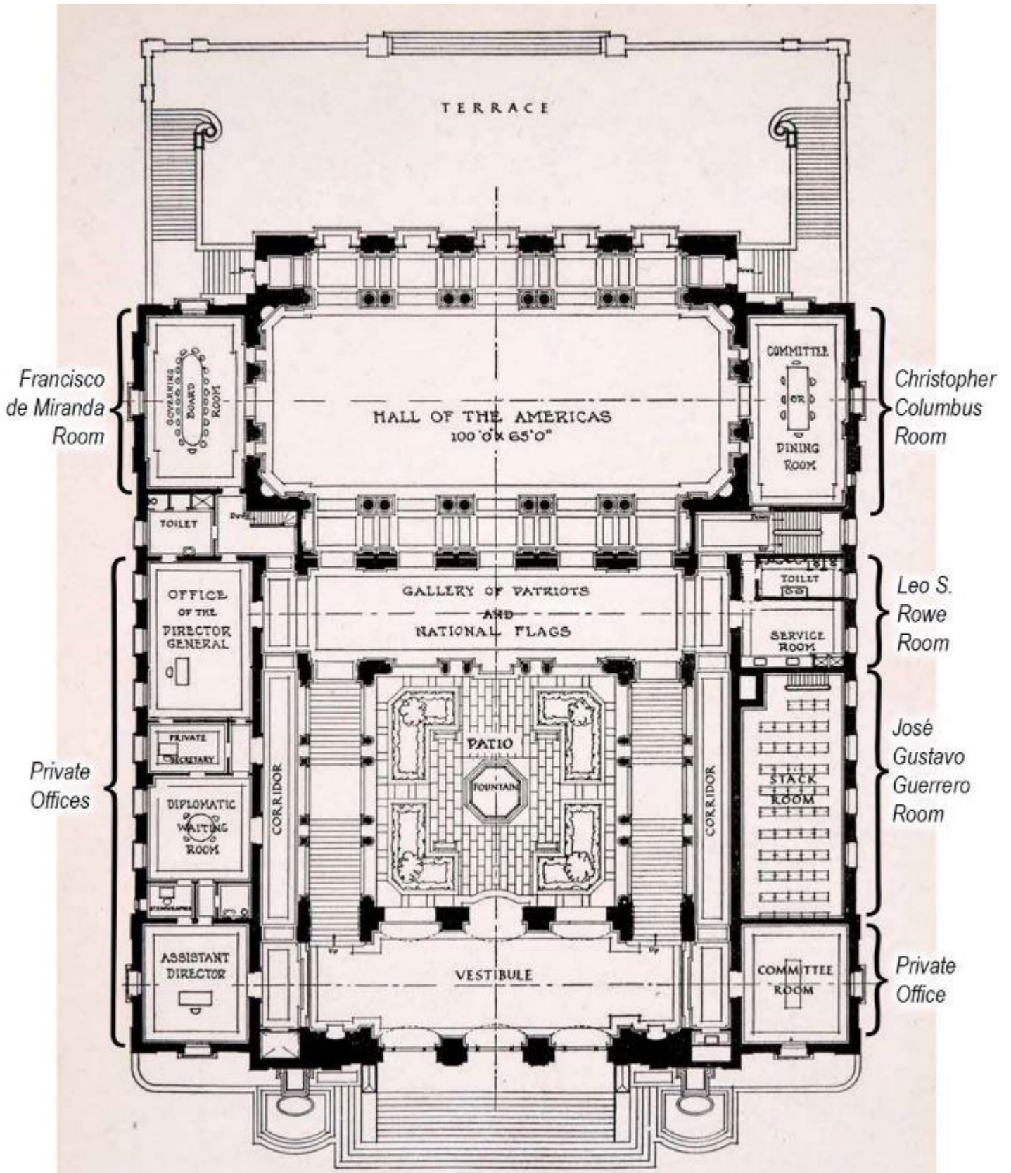
Figure 6: Second floor plan of the Pan American Union Headquarters showing original room designations and current room designations in italics. Source: Barrett, The Pan American Union (1911), 93.
