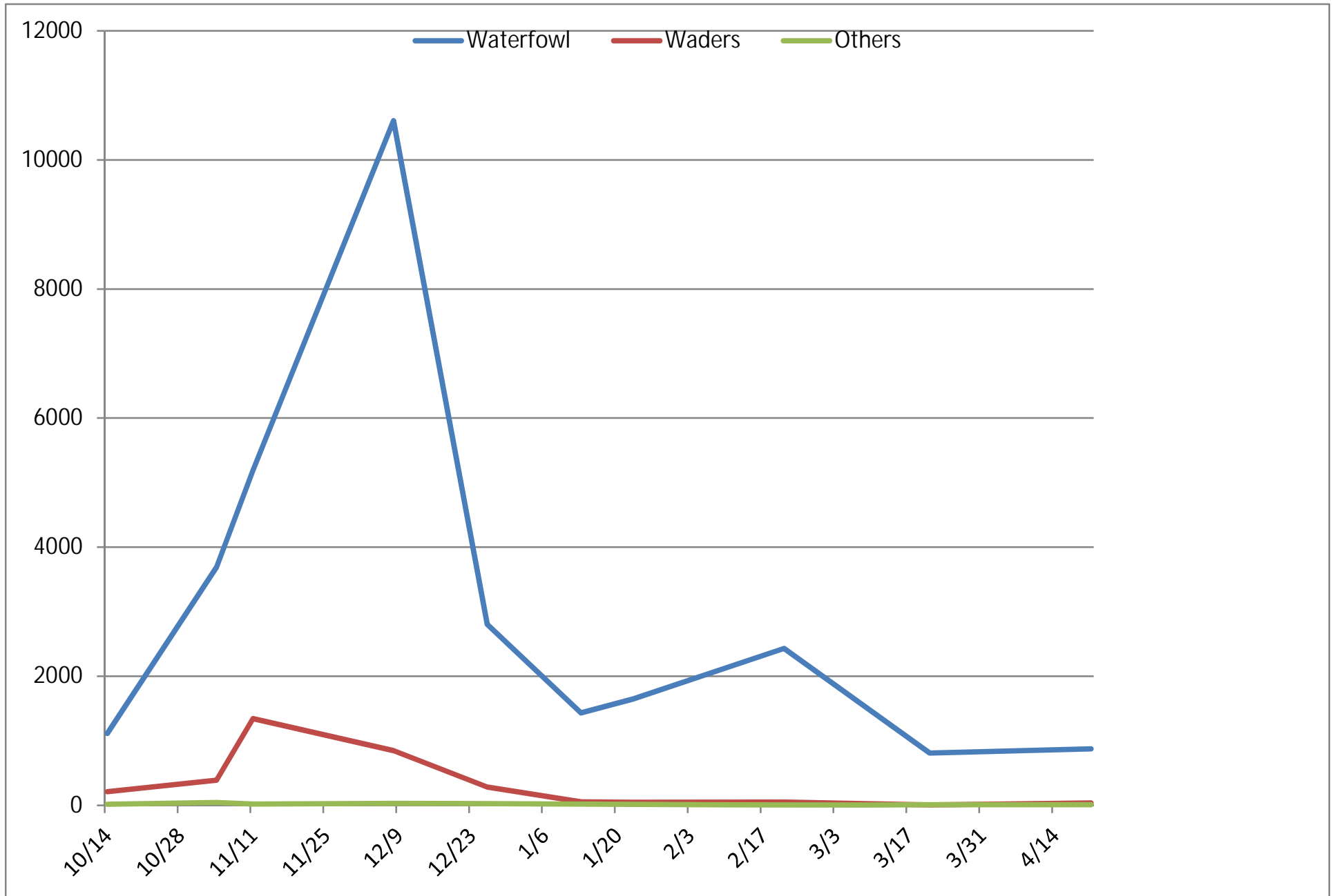
Figure 3. Waterfowl and wader numbers in Year 3, with strong declines in January 2011. Source: Avocet Research Associates.
