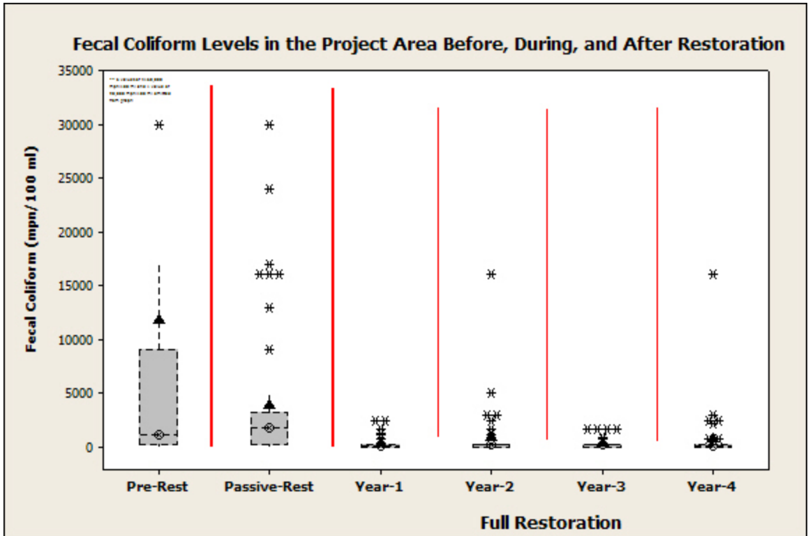
Figure 4. Average, median, and other summary statistics for fecal coliform concentrations for the Project Area Pre-Restoration, during Passive Restoration, and in the first four years of Full Restoration. Note: dashed lines for boxplots indicates both right- and left-censored data. Light-shaded grey boxplots indicate first and third quartiles (25%, 75%), while dark-shaded grey boxplots indicate median confidence intervals. Lines indicate 10 th and 90 th percentiles. Medians are indicated by diagonal-hatched circle, with means designate by black triangles. Note: dashed lines for boxplots indicates both right- and left-censored data.
