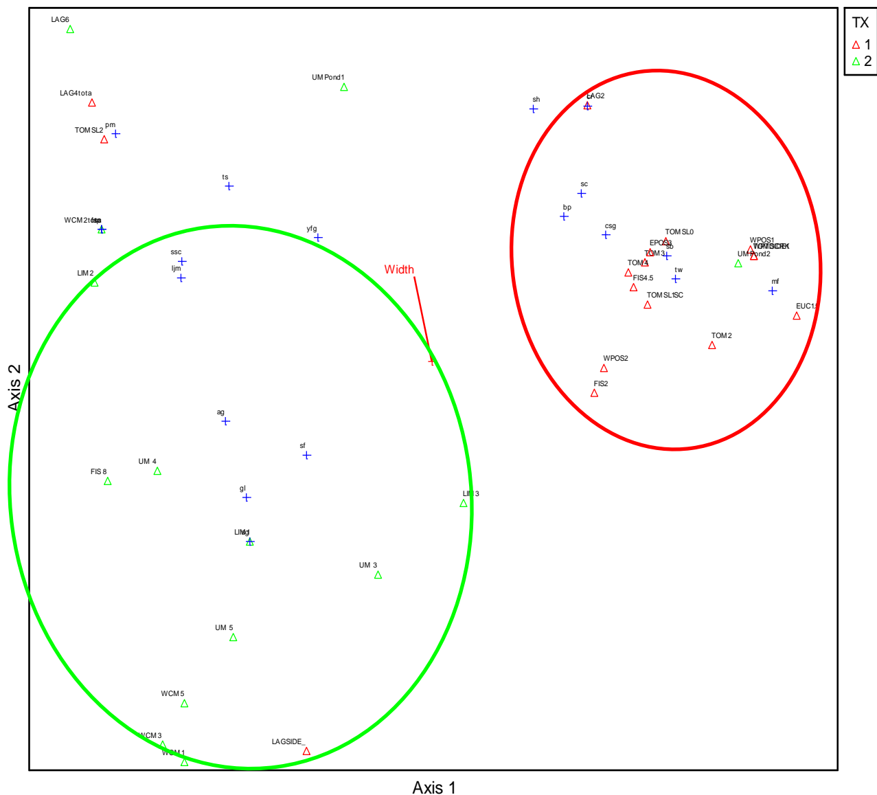
Figure 11. Statistical ordination of fish and macroinvertebrate species assemblages and environmental variables using Non-Metric Multi-Dimensional Scaling (NMDS) between different Study Areas during Full Restoration. There is clear separation between Project Area sites (labeled "1") and Reference Marsh sites (labeled "2"), with width of sampled habitat feature also driving differentiation between sites.
