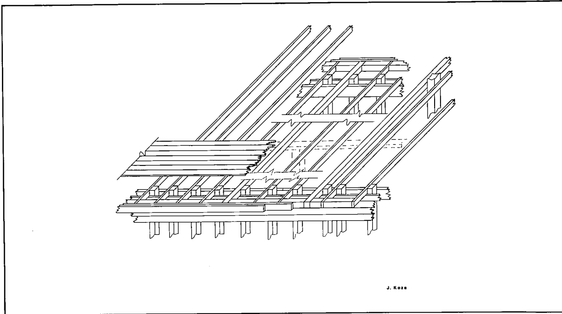
Figure 7.4 Exploded view of main deck construction.
