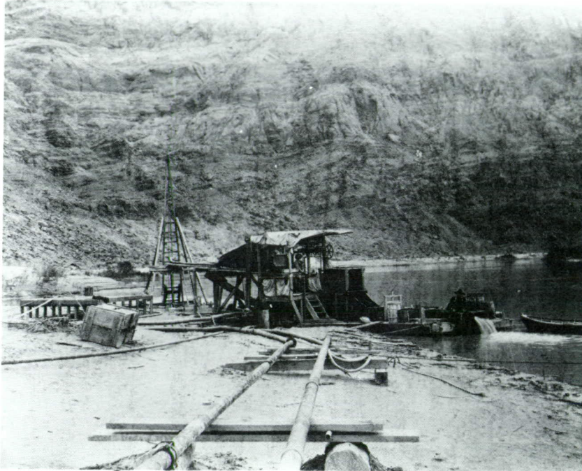
Figure 3.8. The amalgamator at Lee's Ferry. The pipes in the foreground connect the boiler/compressor to the pipe dredge in the left background. From the dredge, the discharged sand was fed to the amalgamator where efforts to extract the gold particles from the sand were carried out. Photo by Emery C. Kolb, November 1911. Special Collections Library, Northern Arizona, Northern Arizona University.
