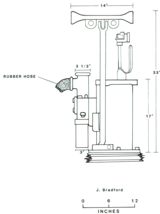
Figure 7.16 Detail drawing of hand-operated bilge pump.
