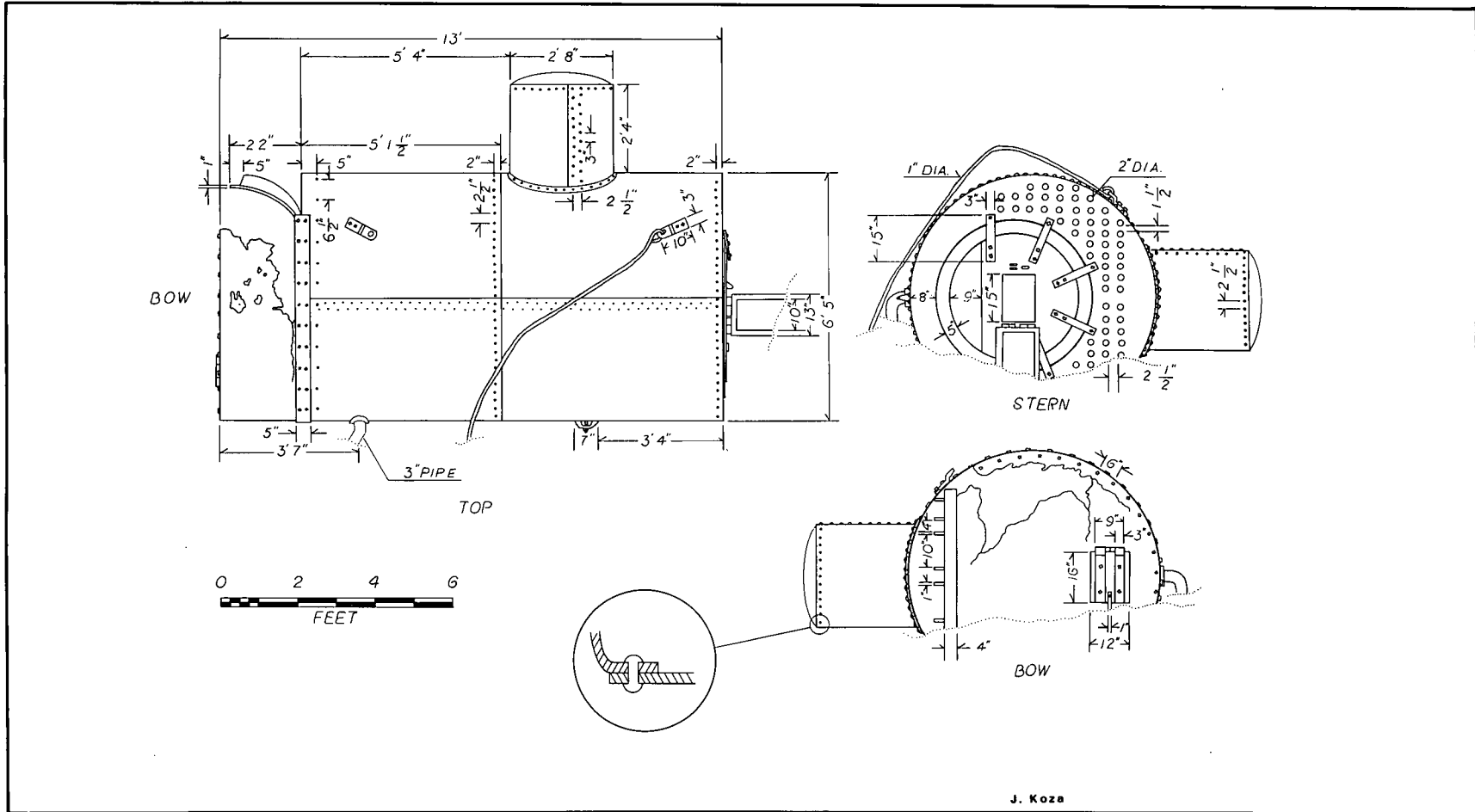
Figure 7.13 Detail drawing of boiler on CHARLES H. SPENCER.
