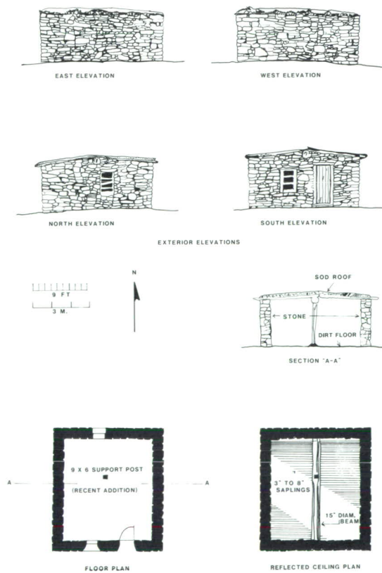
Figure 3.14. Plan and elevation drawings of the post office at Lee's Ferry. The construction methods exhibited in this building are very similar to those used to build the cook's house in 1910. Adapted from Historic American Buildings Survey records.
