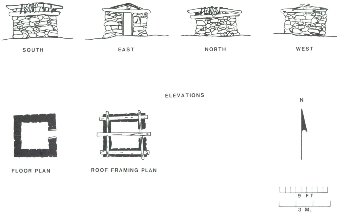
Figure 3.15. Plan and elevation drawings of the chicken coop located northwest of the fort. Adapted from Historic American Buildings Survey records.
