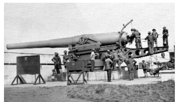
The largest of the new guns installed at the Presidio in the 1890s, like this one at Battery Godfrey, had 12-inch bores.
