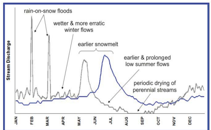
Figure 8. Developing and anticipated changes to the snowmelt flow regime in the Sierra Nevada (gray line), with a more typical historic pattern shown as the blue line. Adapted from David Herbst, Sierra Nevada Aquatic Research Lab.
