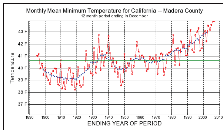
Figure 1. Madera County - the middle among five counties containing SIEN parks, showing Yosemite area minimum temperatures (1895-2007). The blue dotted line is an 11-year running mean. From: Edwards and Redmond (2011).
