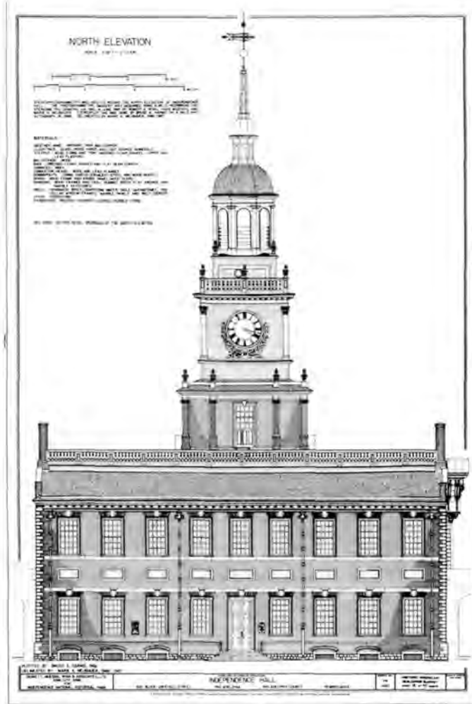
The north elevation of Independence Hall (1733-1750, steeple 1828) shows the main block with the tower rising behind. The drawing shows individual hand made characteristics of the building. Note the sag in the roof, and the variations in the wood board cladding of the tower steeple. In the original drawing the difference between the relieving arches of the cellar windows on either side of the main entrance door can be seen, as well as variations in the Flemish bond brick pattern. Plotted by: Bruce A. Harms, 1986, delineated by: Marie A. Neubauer, 1986-1987 for Independence National Historical Park.
