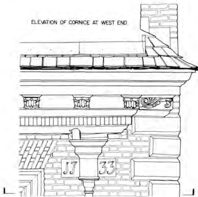
This detail of the west end of the north cornice shows the irregular sizes and shapes of roofing shingles, variations in size and spacing in the dentil course, and the skew of the cornice in relation to the stone quoins at the corner of the building. Plotted by: Bruce A. Harms, 1987, delineated by: Angela J. Schiller, 1988 for Independence National Historical Park.
