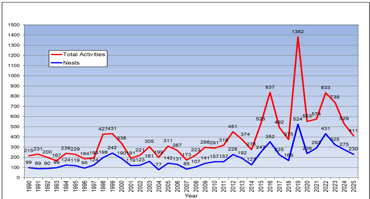
Figure 1. The daily number of nests at 7day increments, May 9 to September 5 and hatchling emergence, July 14 to September 17.
