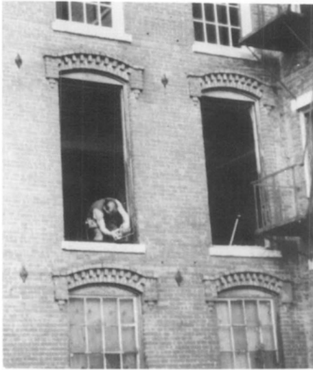
Figure 6. Work on the frames consisted largely of making dutchman repairs to the pulley stiles where required; renailling or replacing brick moldings; replacing some sills; and surface preparation. Photo: Charles Fisher
